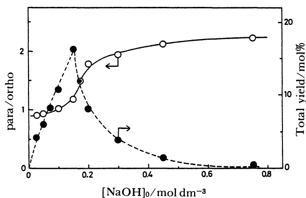
Fig. 1. Plots of the para/ortho ratio (O) and the total yield of 2- and 4-(hydroxymethyl)phenols (●) vs. the charged concentration of sodium hydroxide for the reactions of phenol and formaldehyde in water: [phenol] 0 =0.15 and [HCHO] 0 =0.58 mol dm -3 ; at 30 °C for 1 h.
